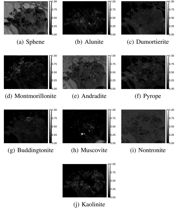
Fig. 7. svvcaBCD/ADMM abundance results (Cuprite scene). The given identification is based on a visual comparison with the results obtained in [28].
