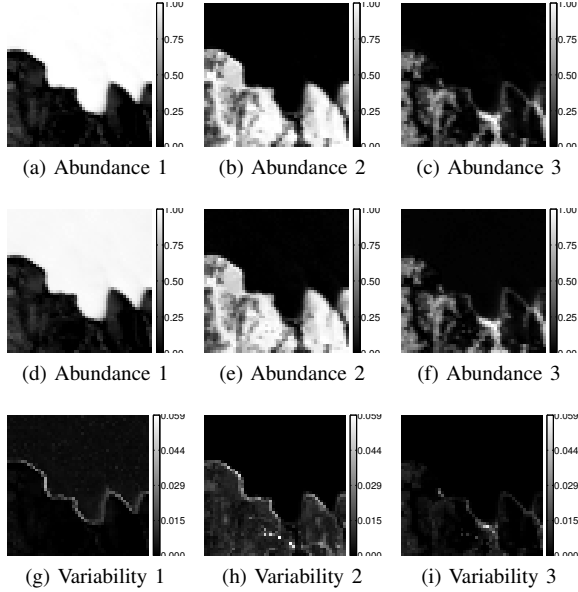
Fig. 5. ssmvBCD/ADMM abundance estimations (Moffett scene). VCA/FCLS results are shown in Figs. 5a to 5c whereas Figs. 5d to 5c are for the ssmvBCD/ADMM. The spatial distribution of the variability with respect to each endmember is presented in terms of energy ( \frac{1}{\sqrt{L}} \|\mathbf{d}\mathbf{m}_{n,k}\|_2 for the k th endmember in the n th pixel) for visualization purpose.
