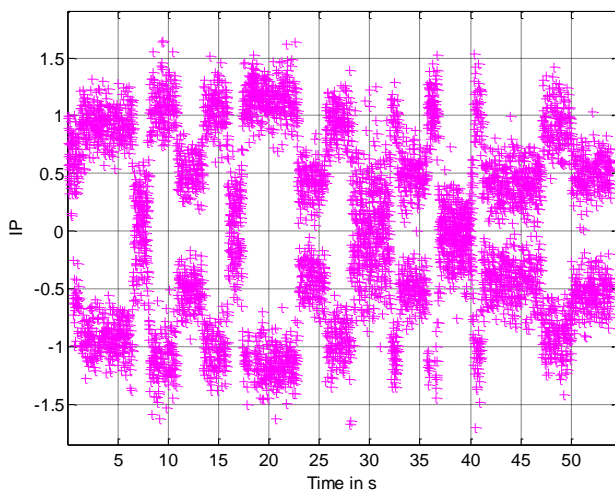
Figure 9: The correlator outputs I_p with the Prieto channel model
