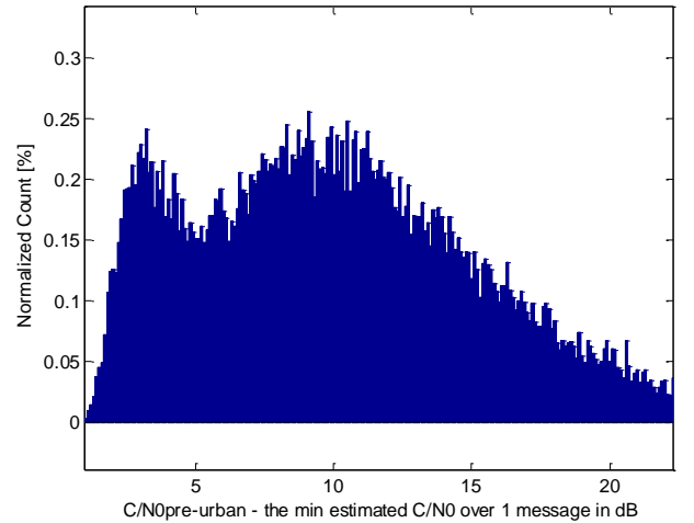
Figure 13: Distribution of the degradation between the C_{\text{pre-urban}}/N_0 value and the minimum estimated received C/N_0 over 1 message, for C_{\text{pre-urban}}/N_0 = 25 dB-Hz and ideal phase estimation with the DLR model
