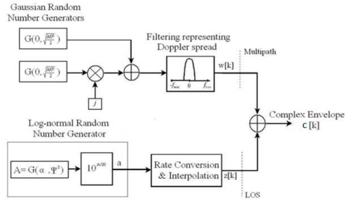
Figure 6: Generation of the c[k] coefficient following a Loo distribution with Butterworth multipath [Burzigotti, 2008]
