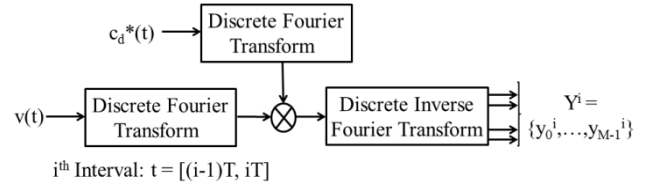
Figure 2: CSK FFT-base demodulator block [11]
