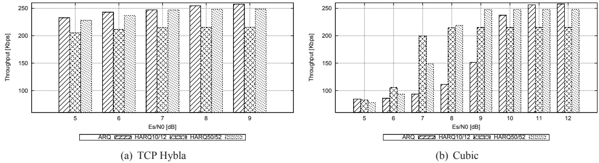
Figure 11: Transport layer performance, without physical layer interleaving
