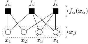
Fig. 1. An example of a factor graph, which is a bipartite graph consisting of variable nodes, (circles/ovals), and factor nodes, (boxes). In this example, \mathbf{x}_a = \{x_1, x_2\} , \mathbf{x}_b = \{x_1, x_3, x_4\} , \mathbf{x}_c = \{x_2, x_3, x_4\} . There are several choices for the inner clusters \mathbf{x}_\beta . One is the full factorization \mathbf{x}_1 = x_1 , \mathbf{x}_2 = x_2 , \mathbf{x}_3 = x_3 , and \mathbf{x}_4 = x_4 . Another is the partial factorization \mathbf{x}_1 = x_1 , \mathbf{x}_2 = x_2 , and \mathbf{x}_3 = \{x_3, x_4\} , which results in the “super node” in the dashed oval. Another is no factorization: \mathbf{x}_1 = \{x_1, x_2, x_3, x_4\} , resulting in the “super node” in the dotted oval. In the latter case, we redefine each factor f_\alpha to have the full domain \mathbf{x} (with trivial dependencies where needed).
